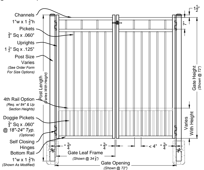
Carolina Double Walk Gate
