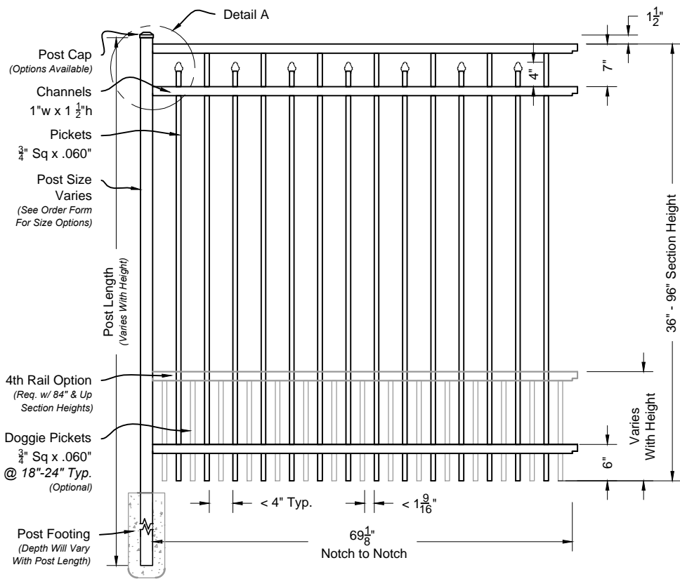
Floridaian #303 6ft Fence Panel Shown As Commercial Series Scale: NTS
