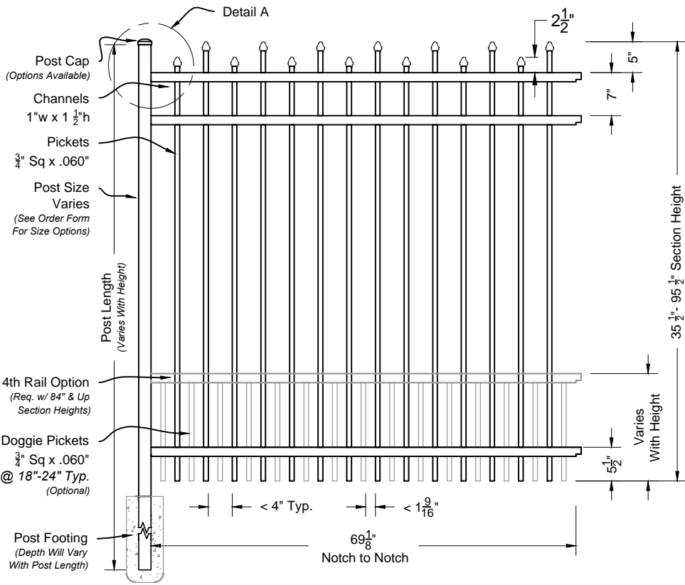
Californian #200 6ft Fence Panel Shown As Commerical Series Scale: NTS
