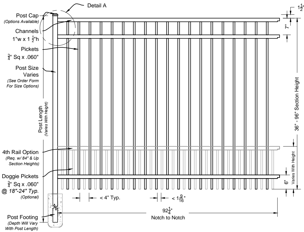
Long Islander #300 8ft Fence Panel
